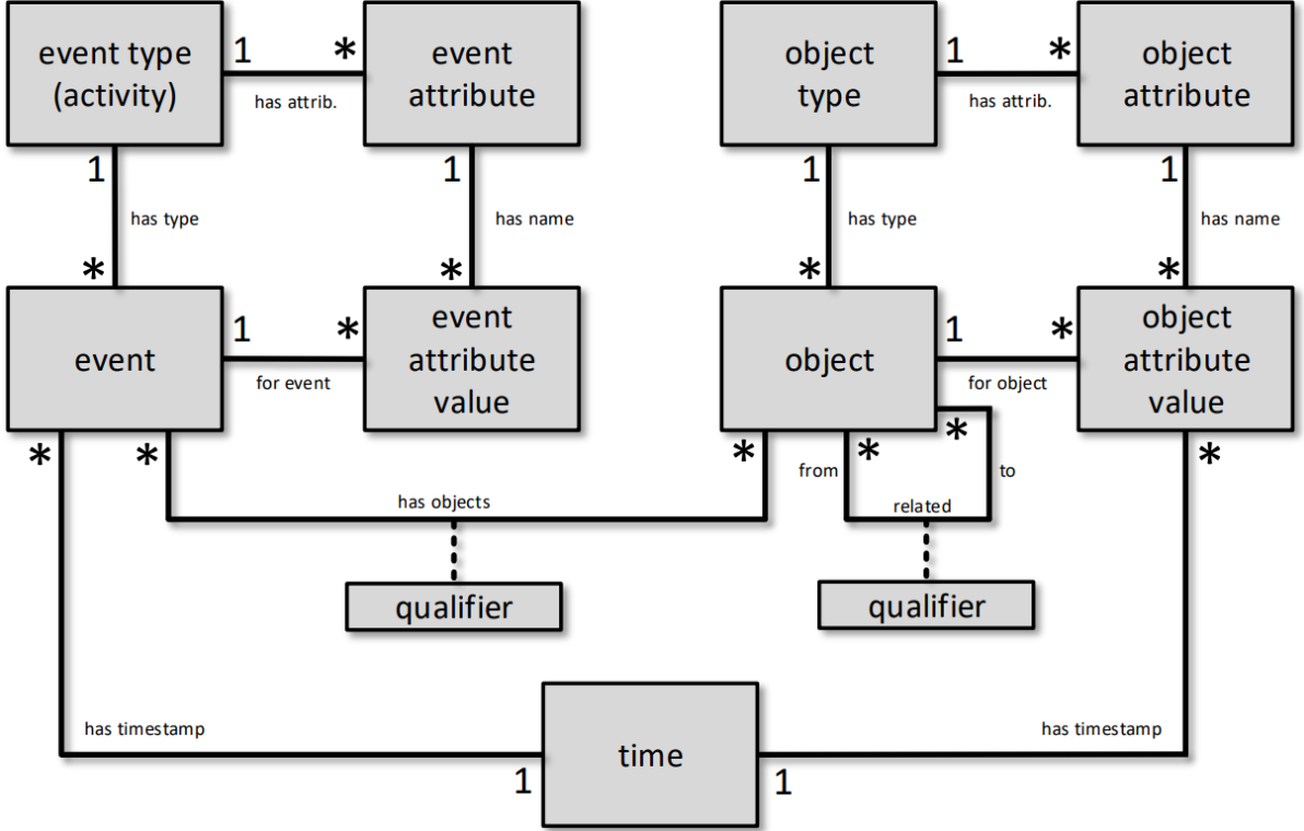
Figure 1: OCEL 2.0 metamodel
